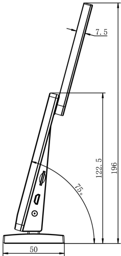
Figure 2: Side view
