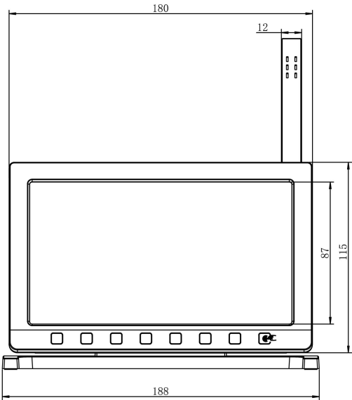
Figure 1: Main view
