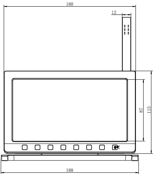
Figure 1: Main view
