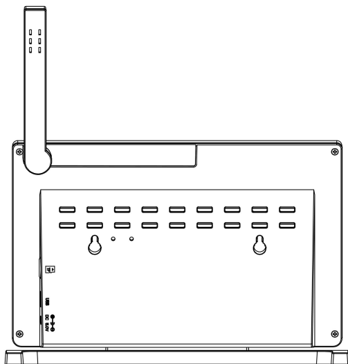
Figure 3: Rear view
