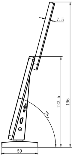
Figure 2: Side view
